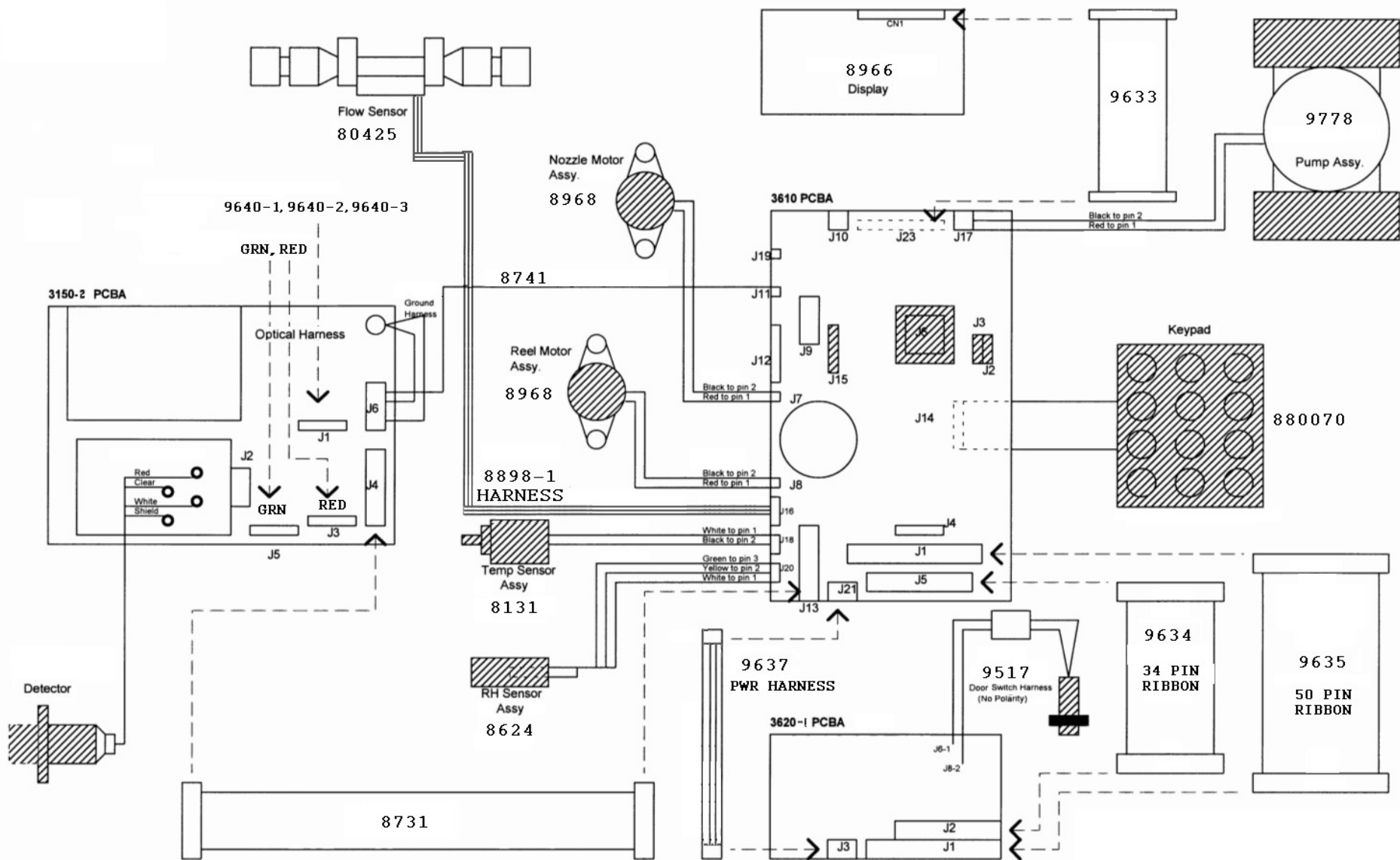
E-BAM INTERNAL, ELECTRICAL INTERCONNECTION DIAGRAM
