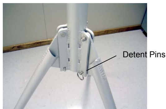
Figure 2-1 Tripod Deployment
