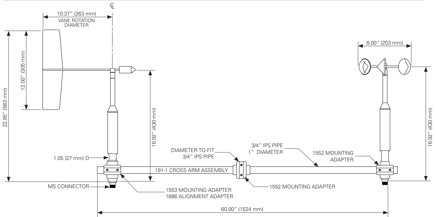
191-1 Mounting Arm & 010C-020C
