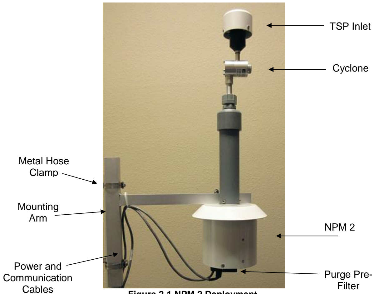
Figure 2-1 NPM 2 Deployment
