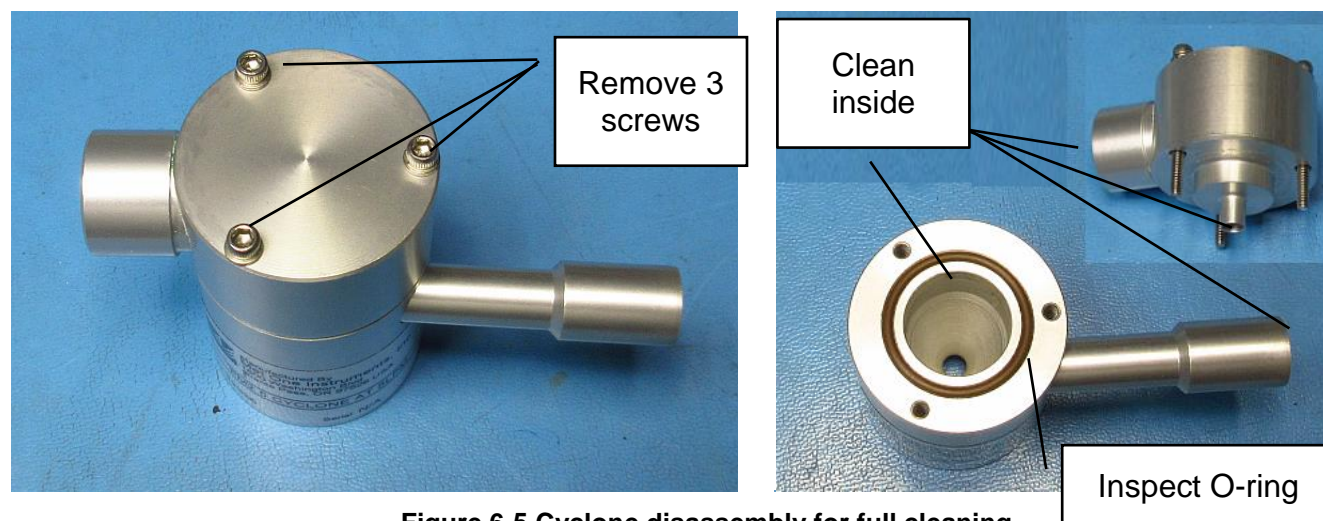
Figure 6-5 Cyclone disassembly for full cleaning
