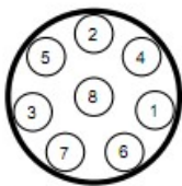
Rear View of Contact Arrangement
