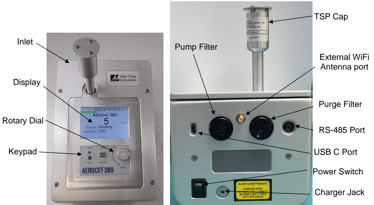
Figure 2-1 - Aerocet-380 Layout
