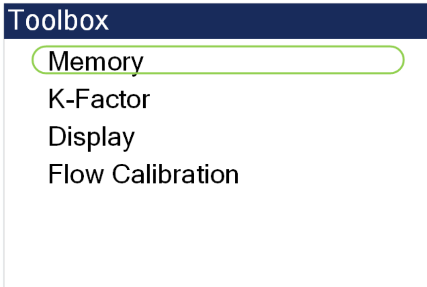
Figure 5-3 - Toolbox Screen
