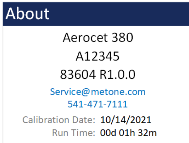
Figure 5-12 - About Screen
