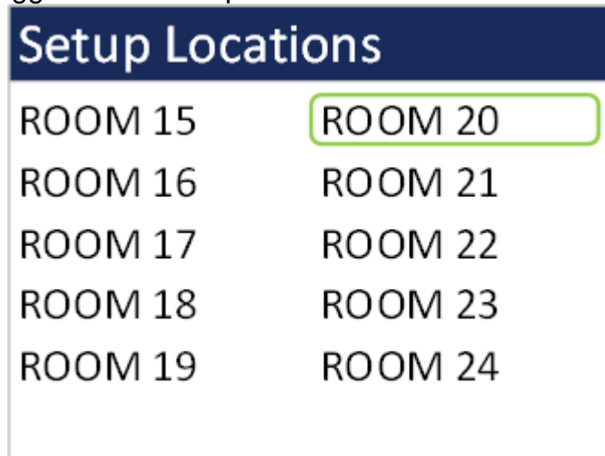
Figure 5-9 - Locations Screen
