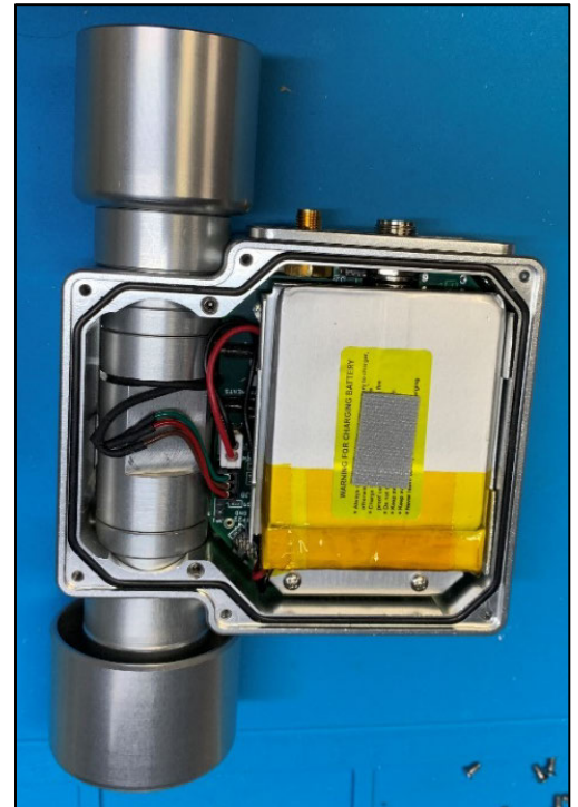
Figure 6-7 Reassembly
