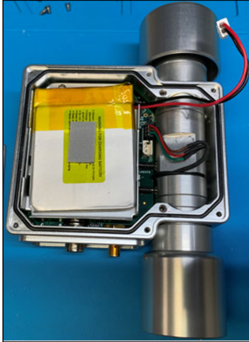
Figure 6-4 Battery Removal
