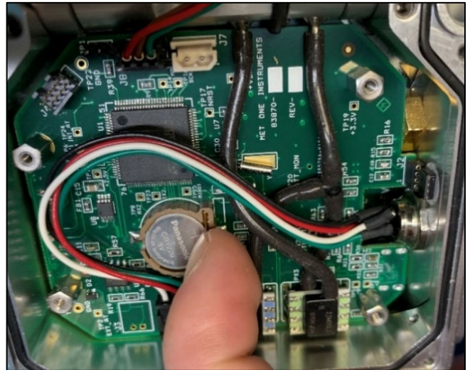
Figure 6-6 Coin Cell Battery
