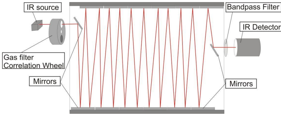
Figure 1 – Measurement Cell Theory
