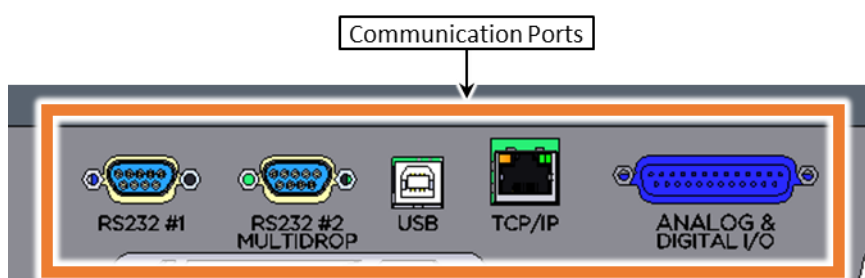
Figure 78 – Communication Ports
