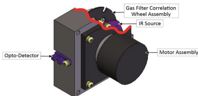
Figure 8 – Source Timing Assembly
