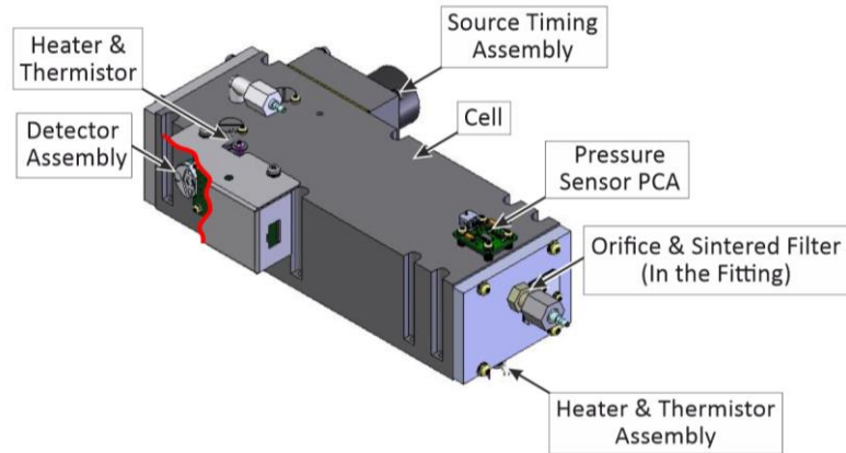
Figure 7 – Measurement Cell
