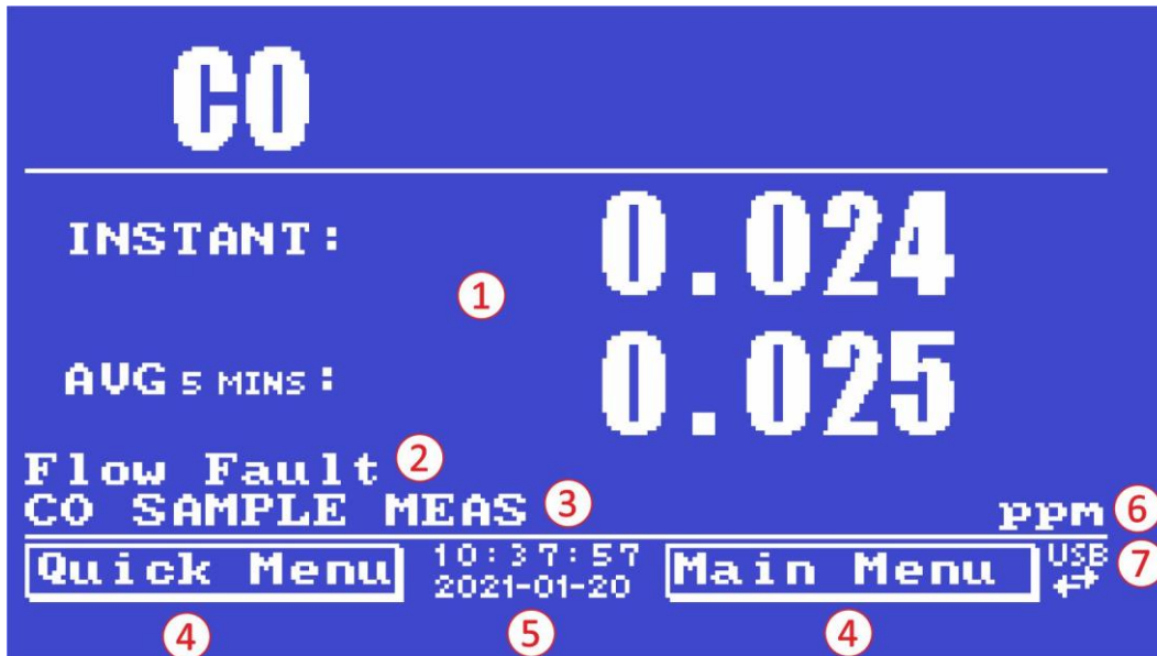
Figure 42 – Home Screen
