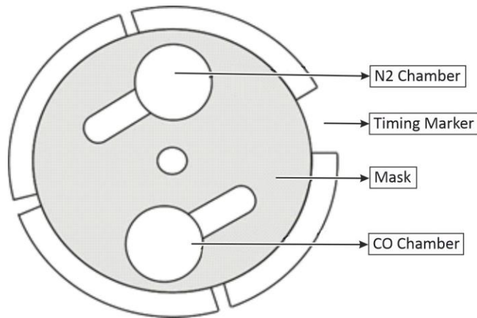
Figure 2 – Correlation Wheel
