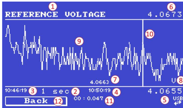
Figure 74 – Chart Screen
