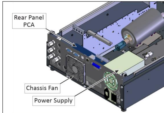
Figure 19 – Rear Panel
